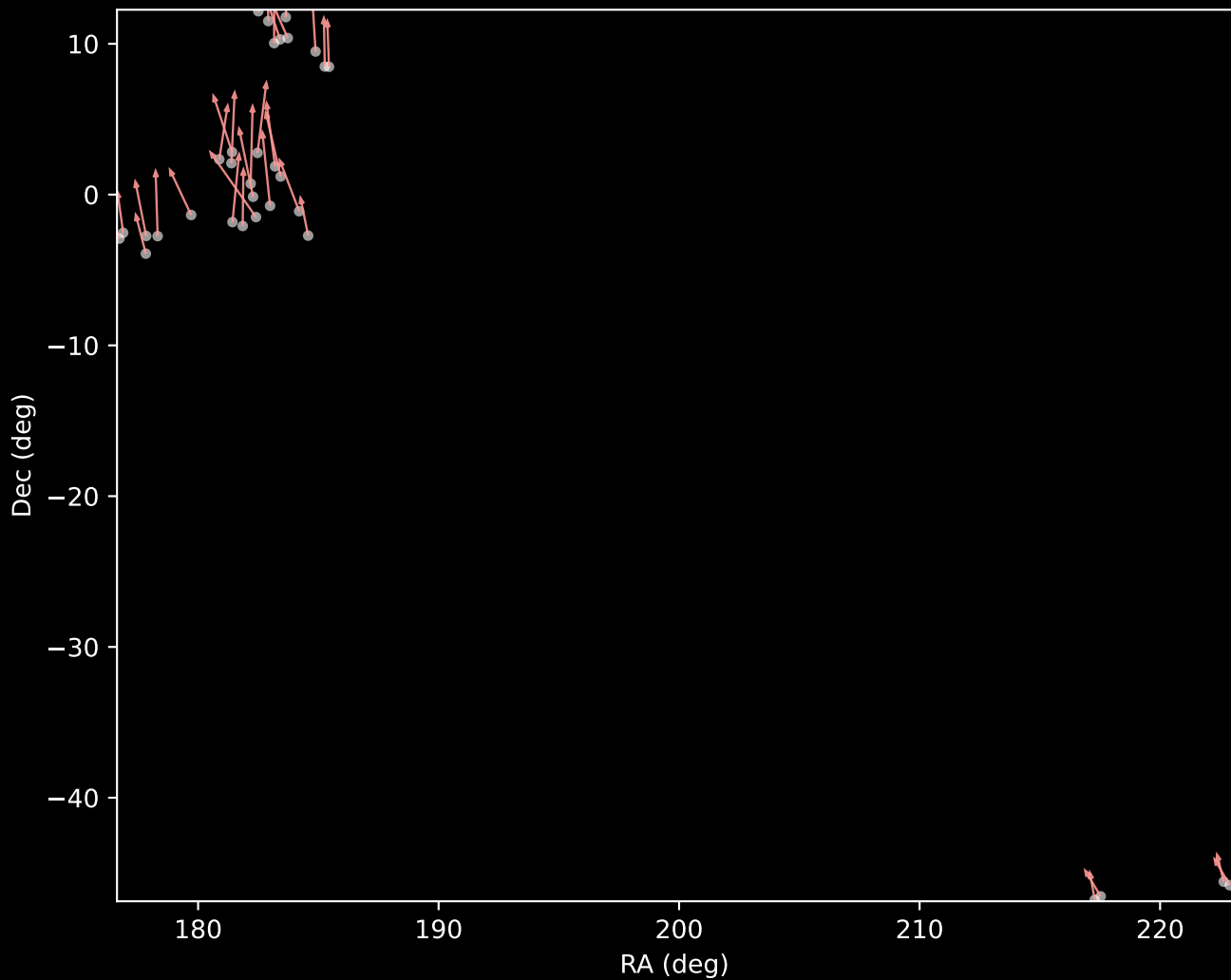
GALAH DR4 Cluster 27 Proper Motion Vectors (n=33)
