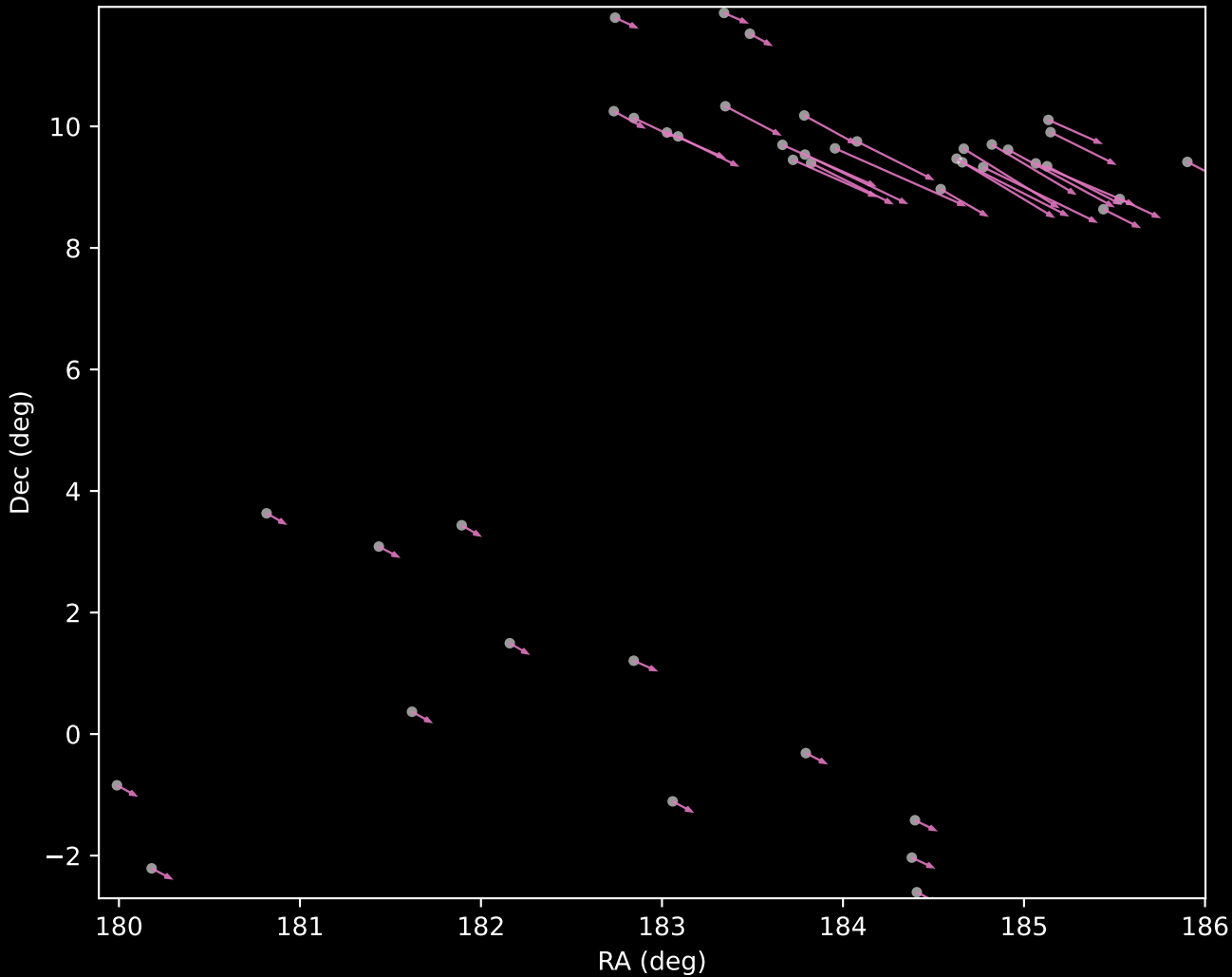
GALAH DR4 Cluster 192 Proper Motion Vectors (n=42)
