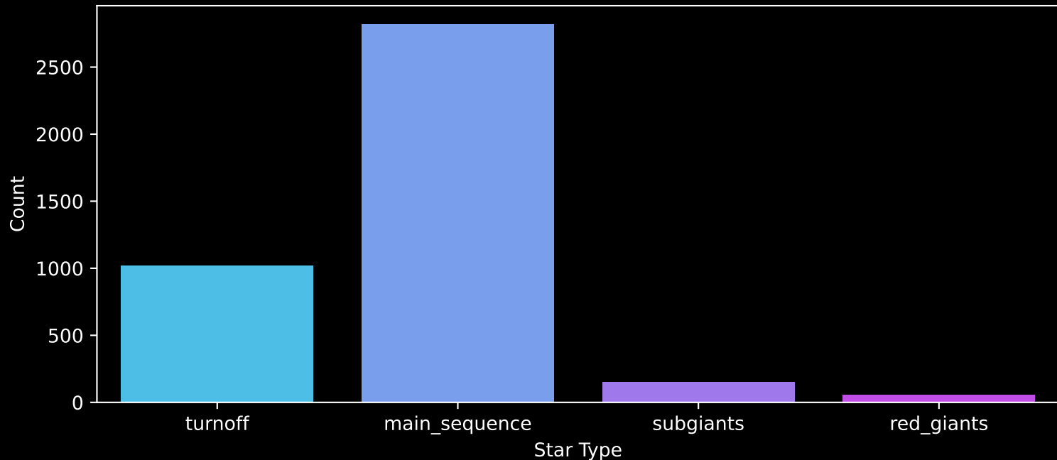
GALAH DR4 Field: [-8] Count plot of Star Type
