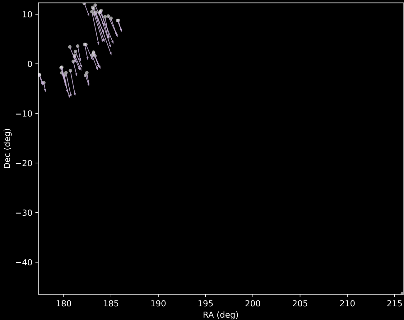
GALAH DR4 Cluster 129 Proper Motion Vectors (n=39)
