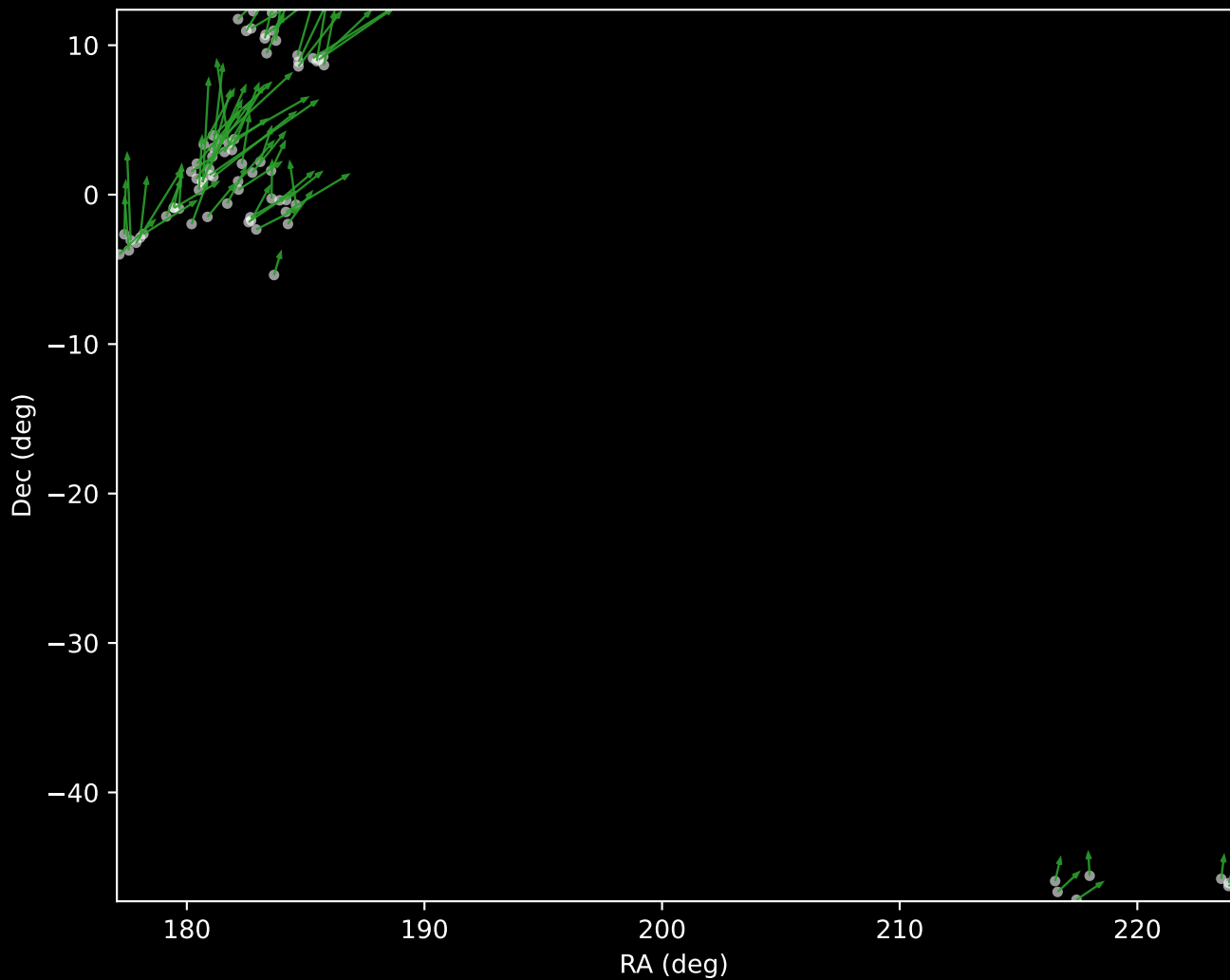
GALAH DR4 Cluster 44 Proper Motion Vectors (n=74)
