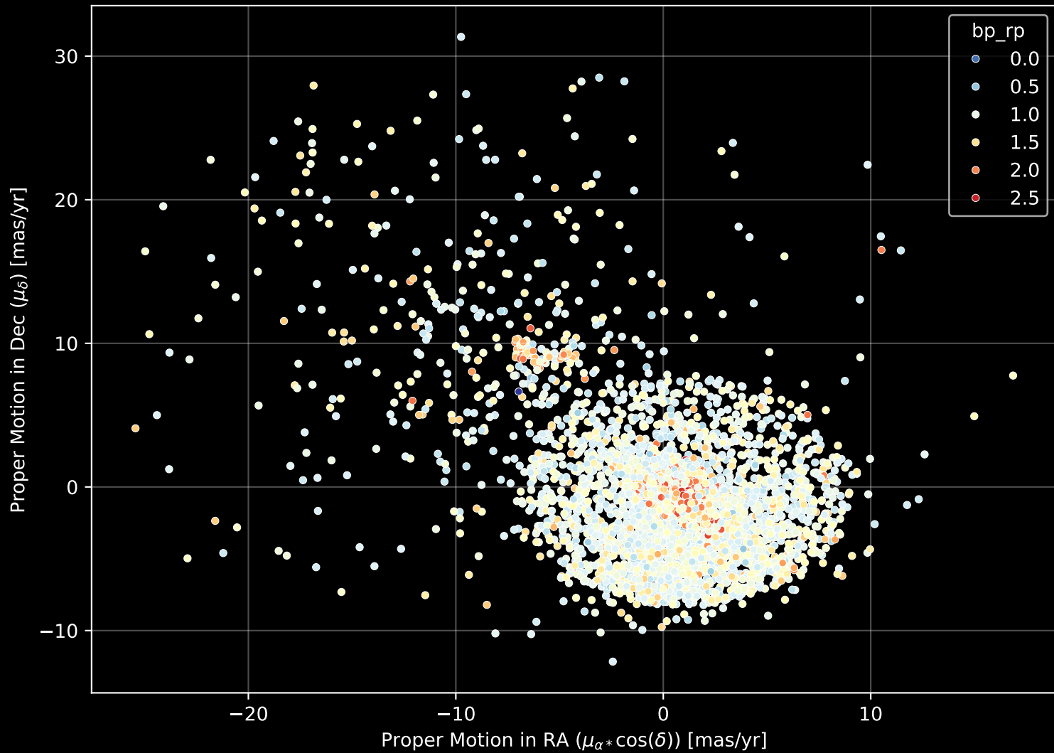
GALAH DR4 Field: [-8] Proper Motion Diagram (n= 4043)
