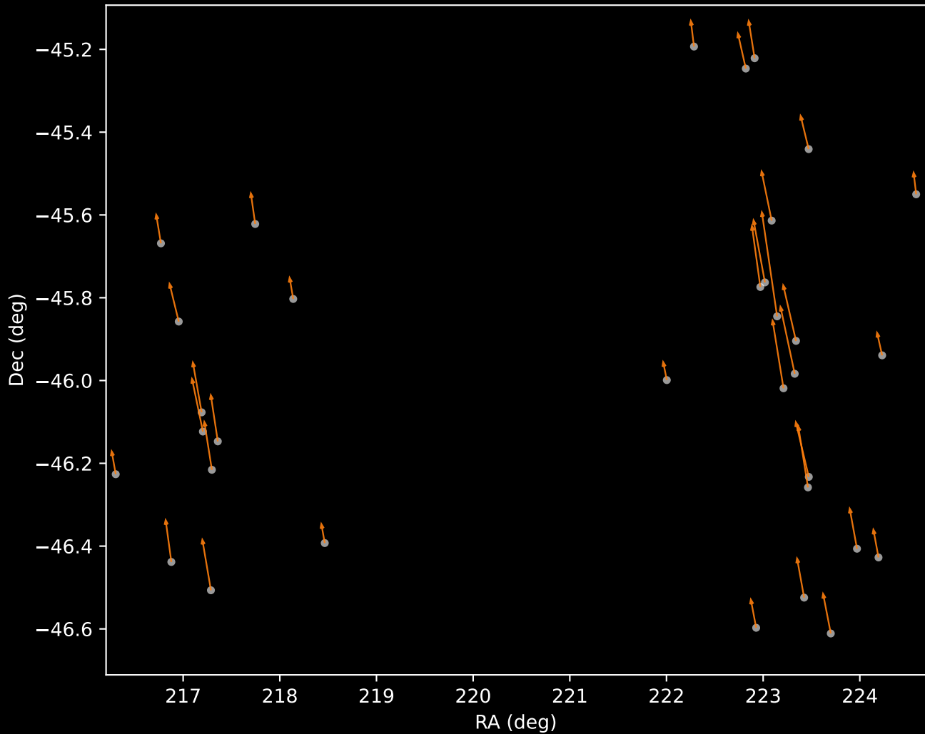
GALAH DR4 Cluster 2 Proper Motion Vectors (n=33)
