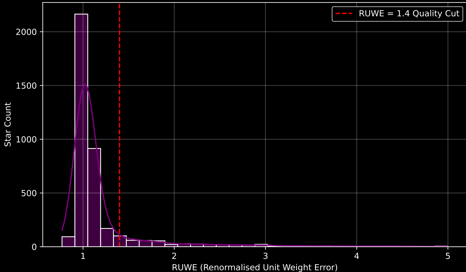
GALAH DR4 Field [-8] RUWE Distribution (n= 3876)
